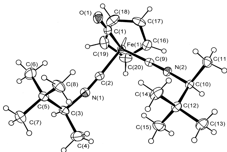
Figure 1. ORTEP view of the cationic part of carbonylcyclopentadienyldi[( S )-1,2,2-trimethylpropylisocyanide]iron(II) hexafluorophosphate, 16 . Ellipsoids at the 50% probability level.
